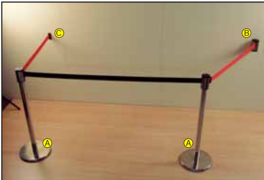
A BELT STAND AP1715 Base dia: 350mm Pole height: 1000mm
